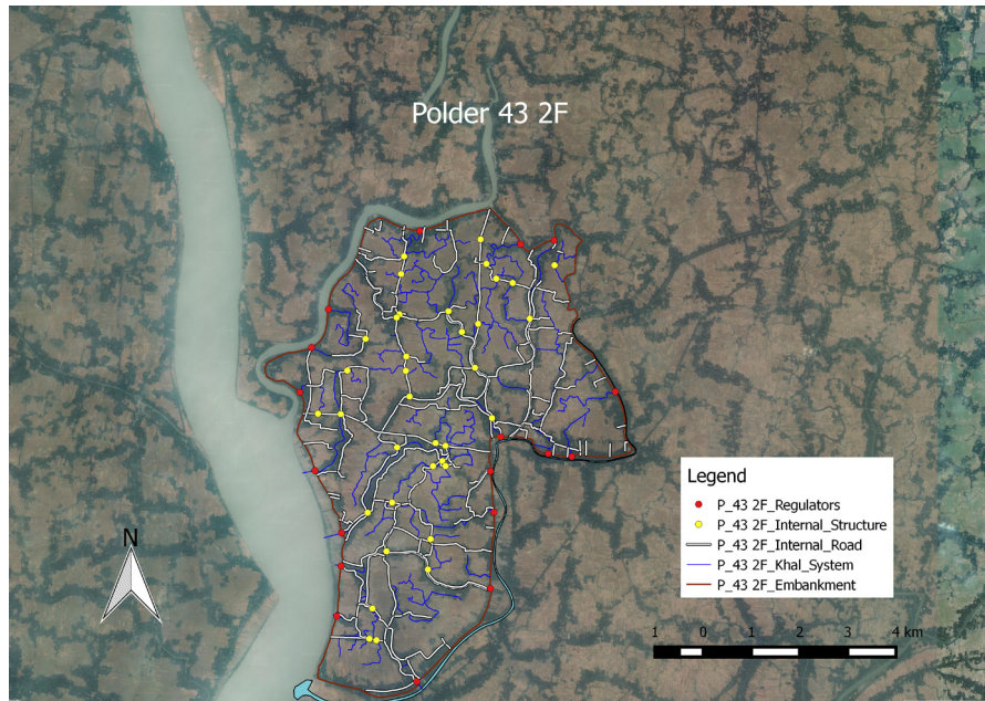
Figure 12 Polder 43 2F: Physical infrastructures.
