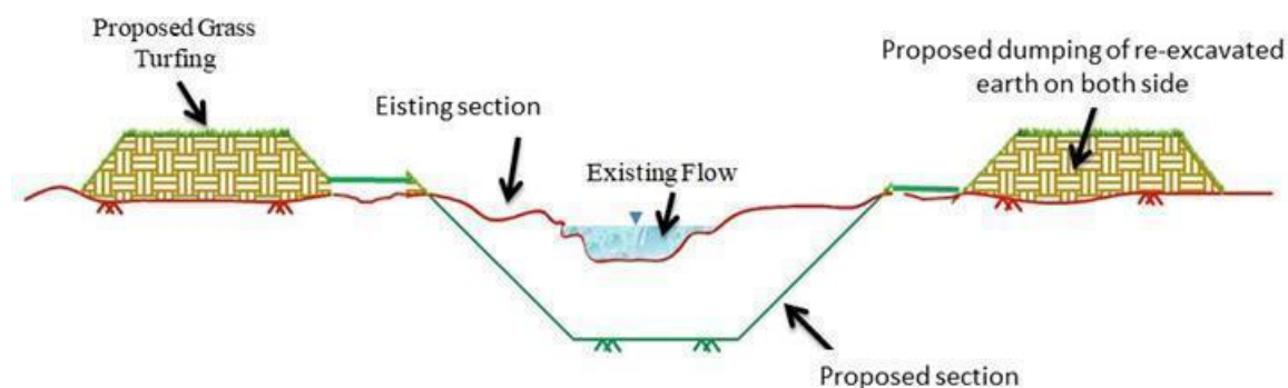
Figure 0.3 Conceptual Cross Section of a typical khal to be re-excavated
