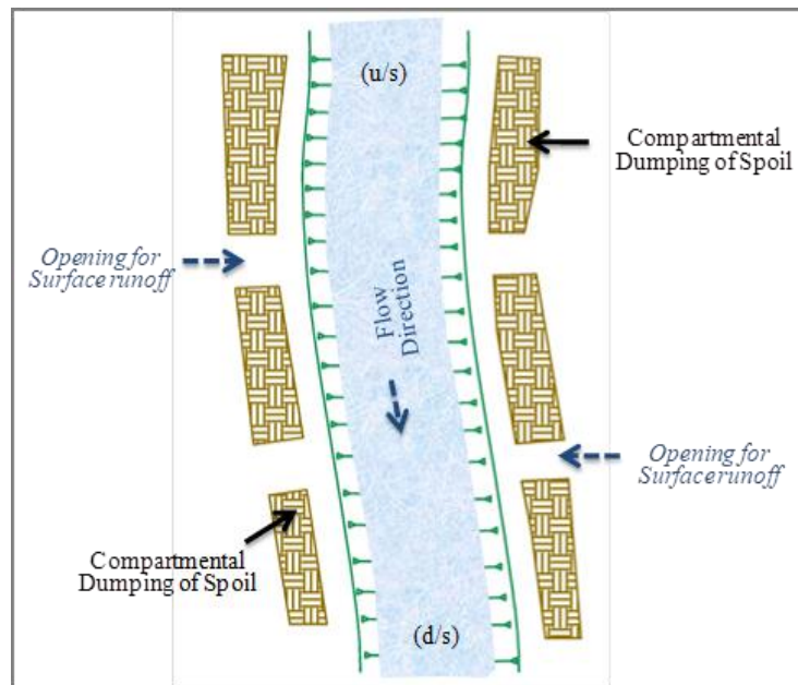
Figure 0.4 Plan form of a typical khal to be re-excavated
