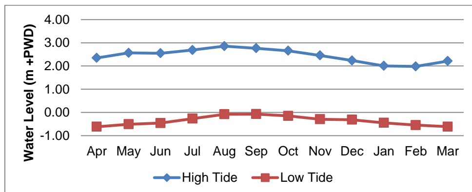
Figure 5.9 Surface Water Level at Chalna (Rupsa-Pasur River)
